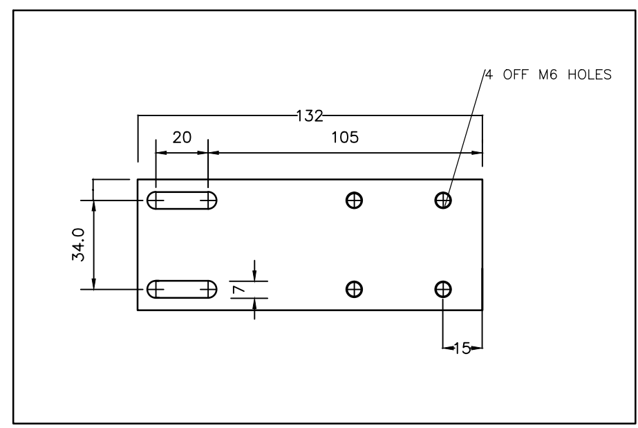
294-22520 Angle 2x2" (1)
