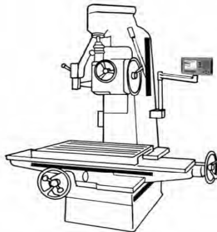
FIGURE 4.1 Jig Borer
